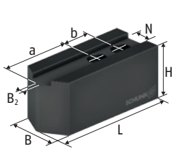
SWBL 软顶爪
