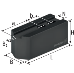
SWBL 软顶爪
