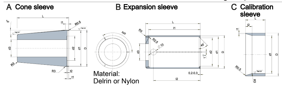
Assembly tools for the piston seal
