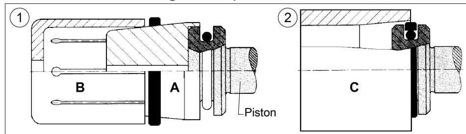
Assembling the piston seal
