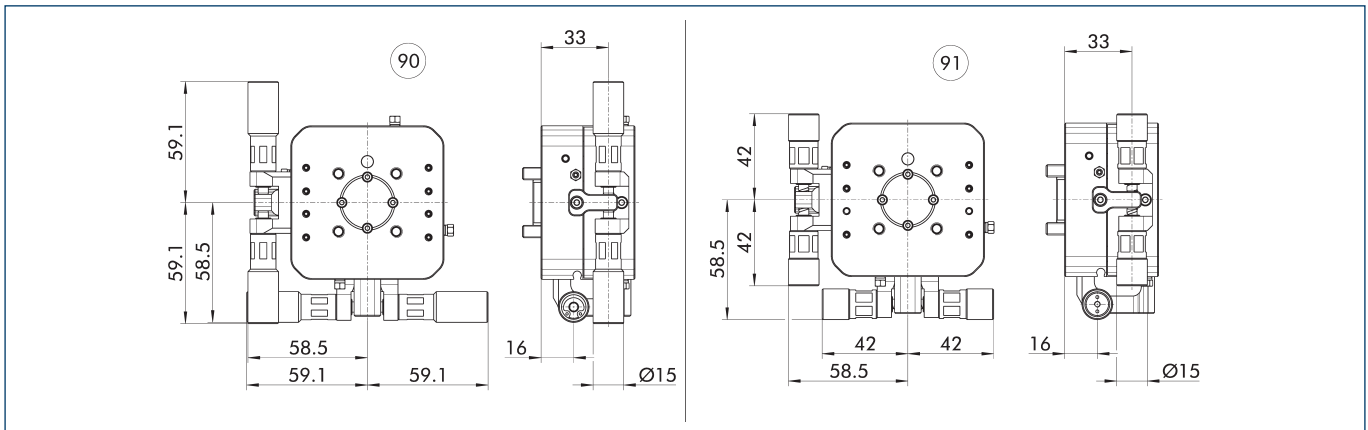
90 Federpatrone (FP)
