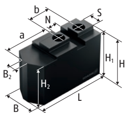
SRK 软顶爪
