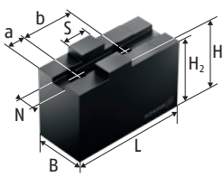
SFA 软顶爪
