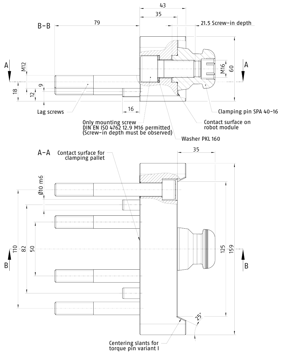
PKL 160 Lean pallet coupling
