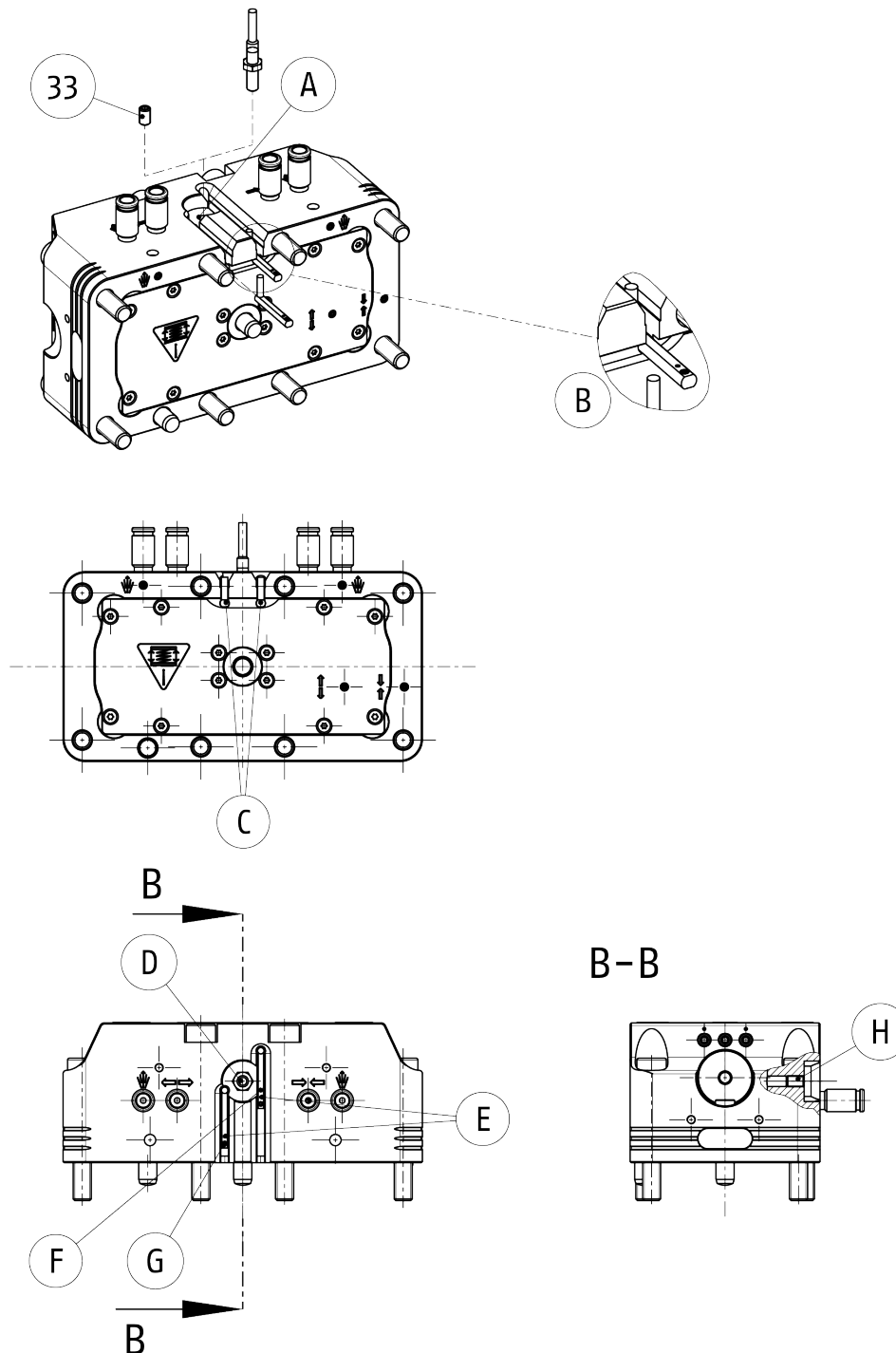
Mounting the proximity switches on the NSR3 160-84
