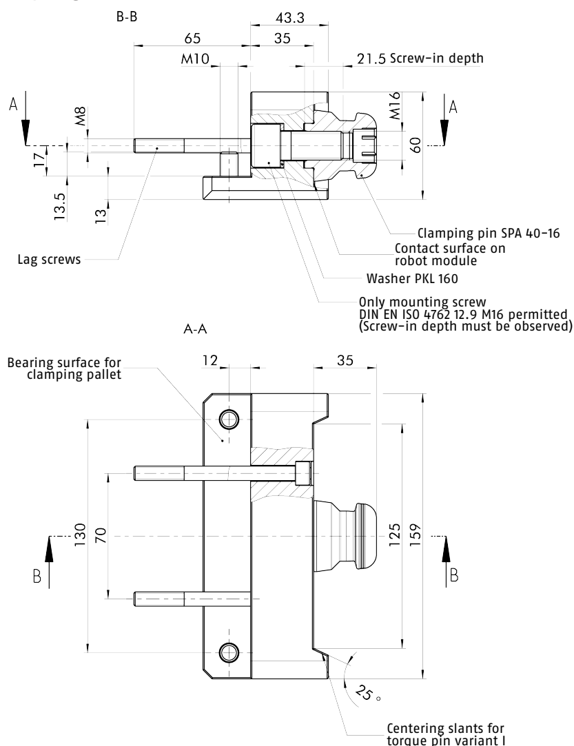
PKL-K 160 pallet coupling (PKL 160 interface identical)
