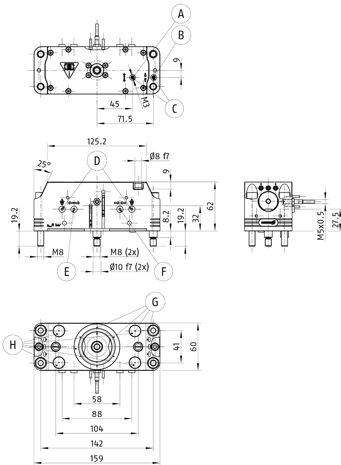
Mounting and connections NSR3 160
