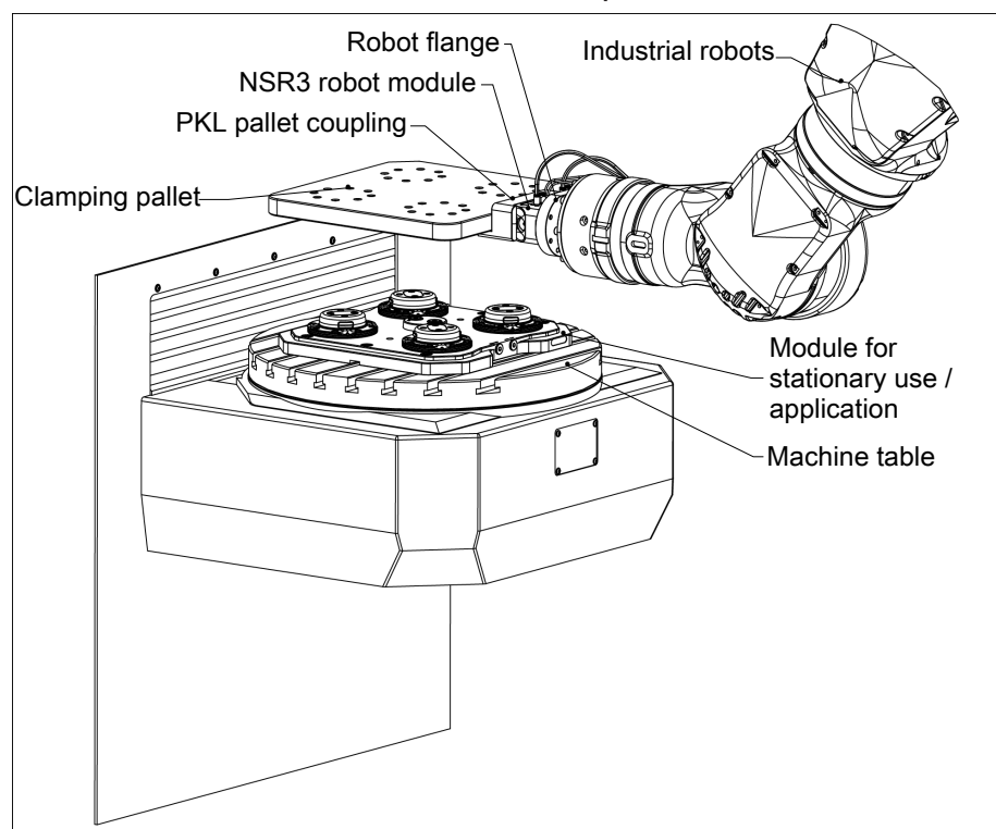
Application example for automated pallet loading
