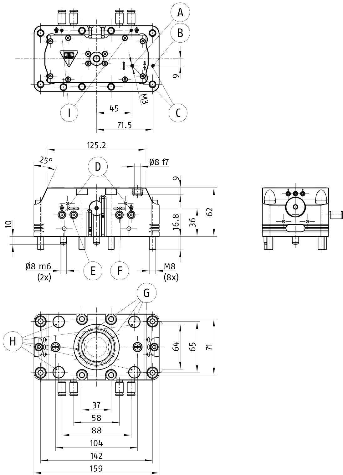
Mounting and connections NSR3 160-84
