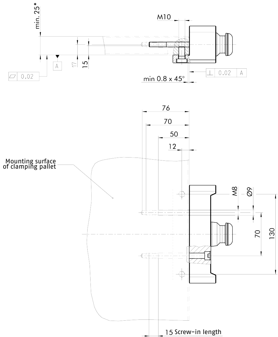
Connection interface between the clamping pallet and pallet coupling (PKL-K 160, PKL 160)
