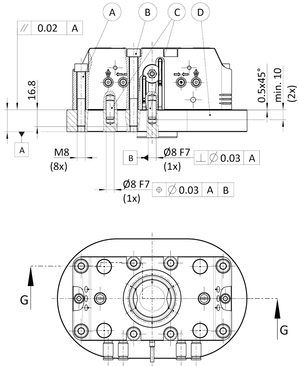
Mounting NSR3 160-84
