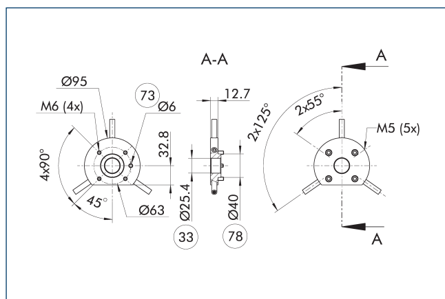
Plaque interface CTS C-025-AH-CPS020-021
