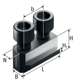
NK Nutenstein
