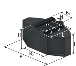
SWB-SM Segmentbacken
