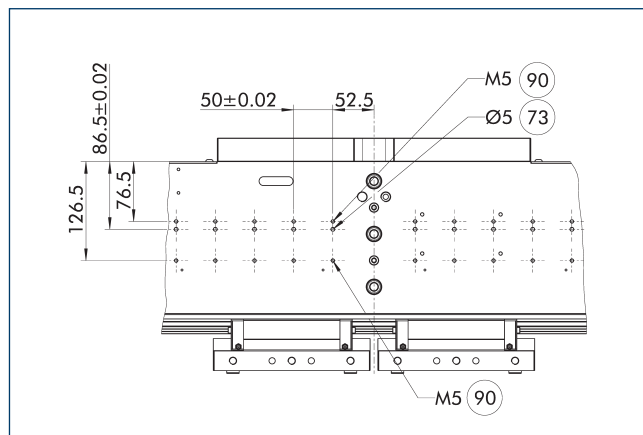
73 适合定心销
