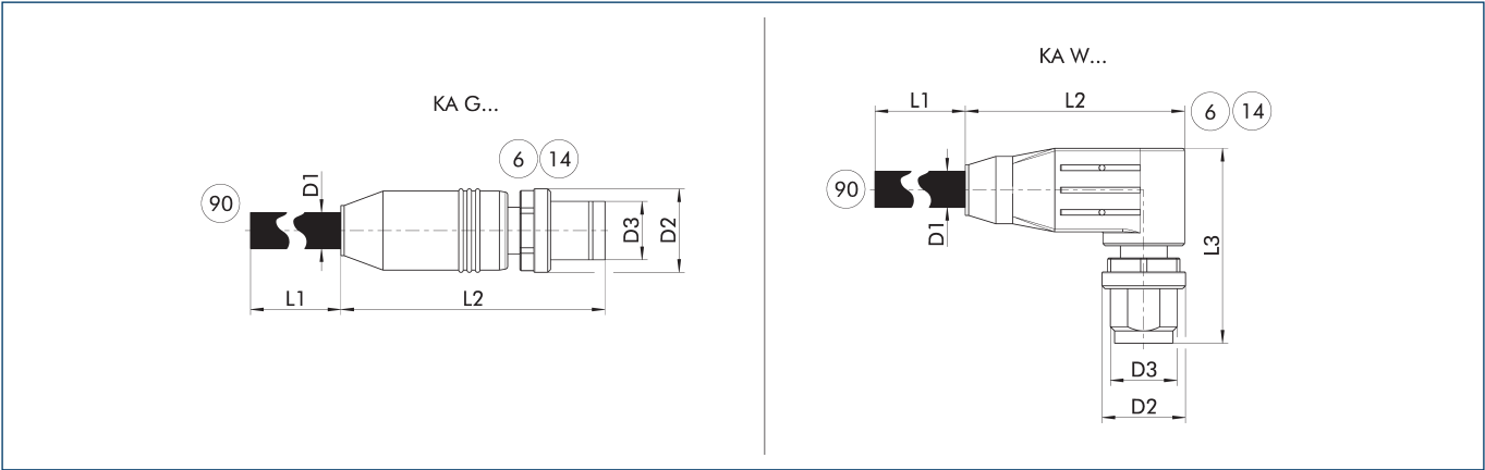
KA G... Straight plug connector ⑥ Connection module side ⑨⑩ Cable ends with second plug connector KA W... Angular plug connector ⑮ Connector
