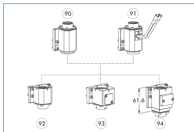
90 SWO-S26-K
