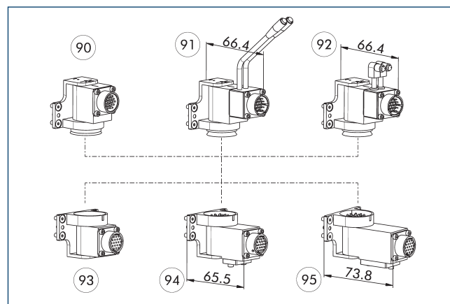
90 SWO-G19-K
