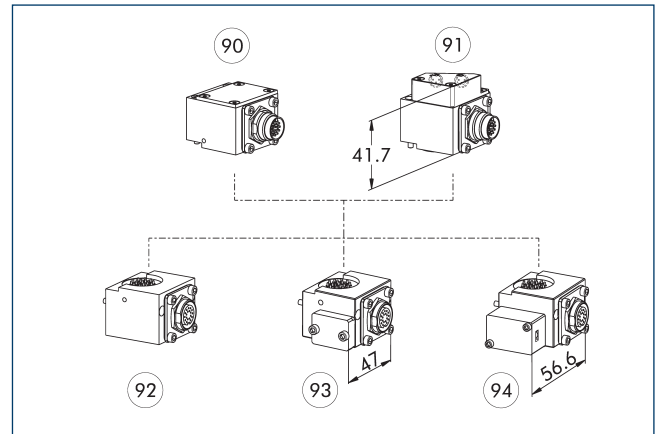
90 SWO-KF19-K
