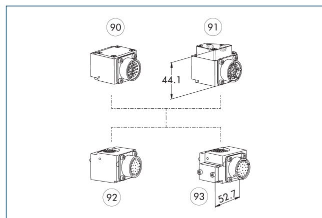
90 SWO-K26-K
