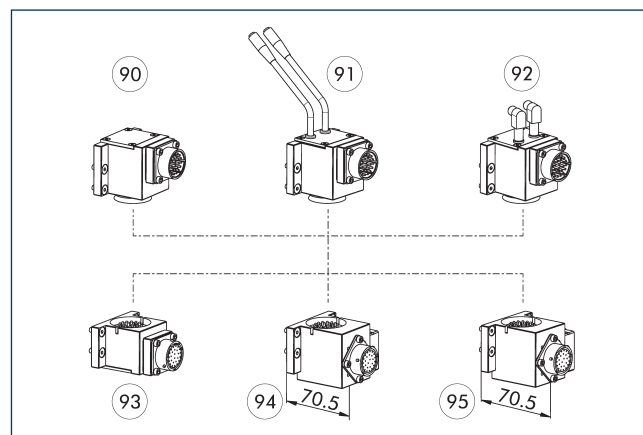
90 SWO-R26-K
