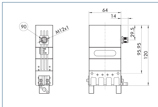
90 M12, 5-pin
