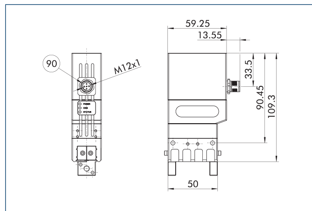
⑨⑩ M12, 5-pin
