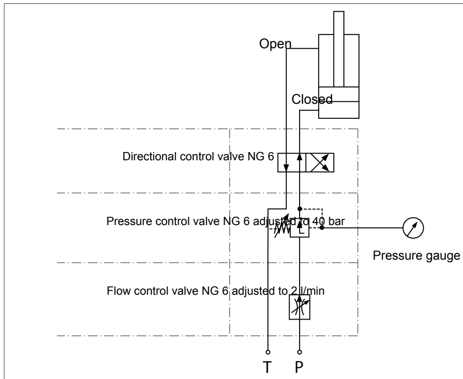
Wiring diagram
