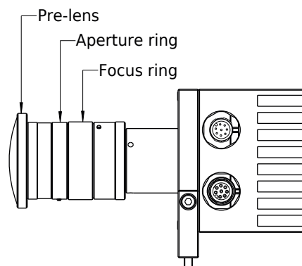
Fig. 4.3: Focus and aperture rings on the rc_randomdot White
