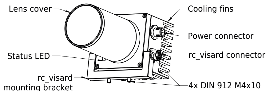
Fig. 3.1: Parts description
