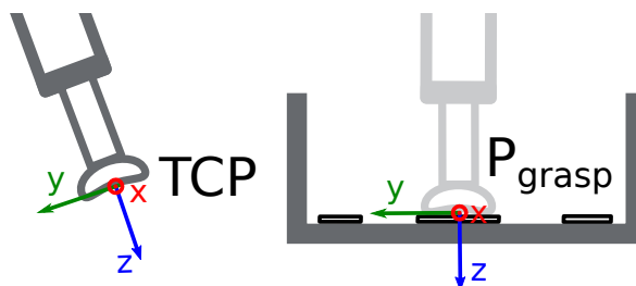
Fig. 7.3: Definition of grasp points with respect to the robot's TCP
