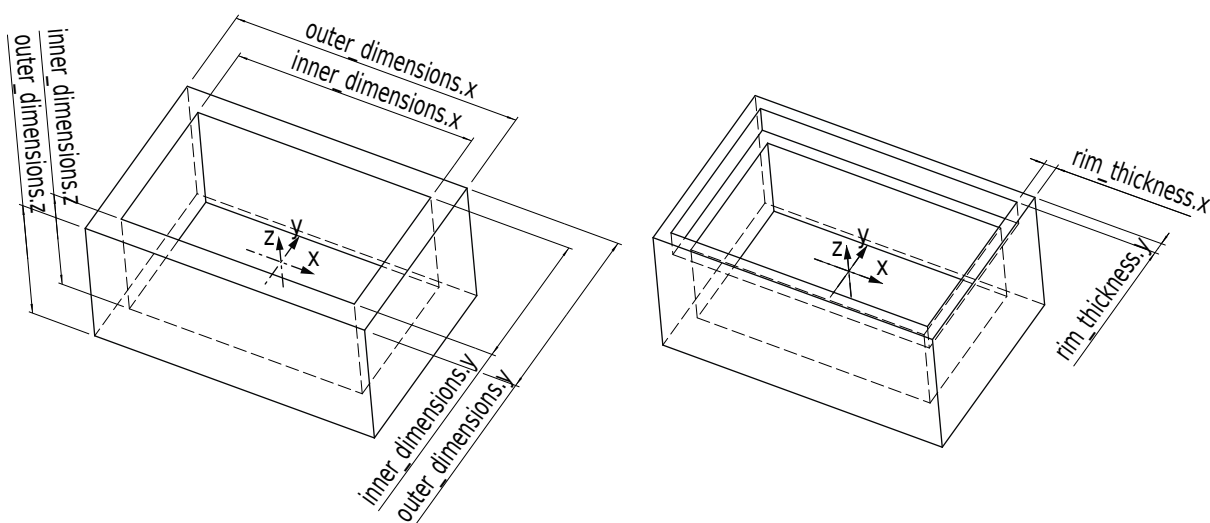
Fig. 7.10: Load carrier models and reference frame
