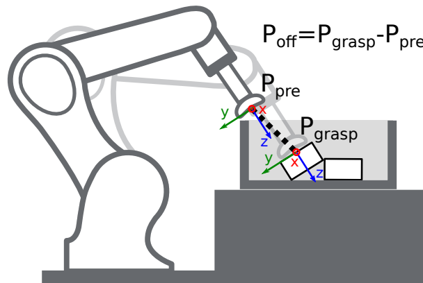
Fig. 7.7: Illustration of the pre-grasp offset parameter for collision checking. In this case, the pre-grasp position as well as the grasp position are collision free. However, the trajectory between these poses would have collisions. Thus, this grasp pose would be marked as colliding.
