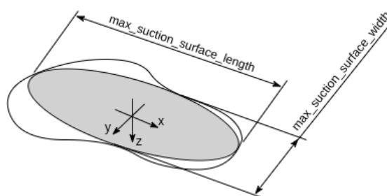
Fig. 7.2: Illustration of suction grasp with coordinate system and ellipse representing the maximum suction surface.
