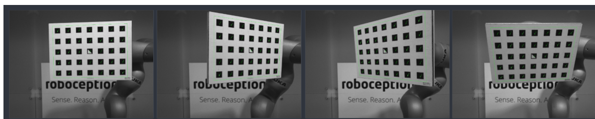
Fig. 6.25: Recorded close view camera images as input for the calibration procedure
