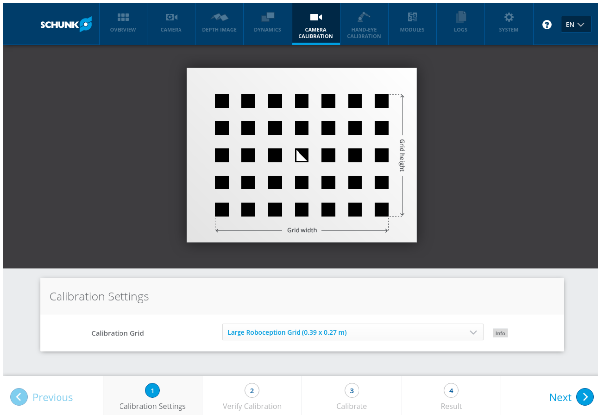
Fig. 6.9: Calibration settings
