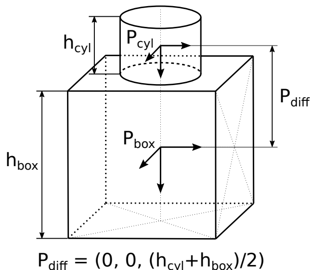
Fig. 7.6: Reference frames for gripper creation via the REST-API
