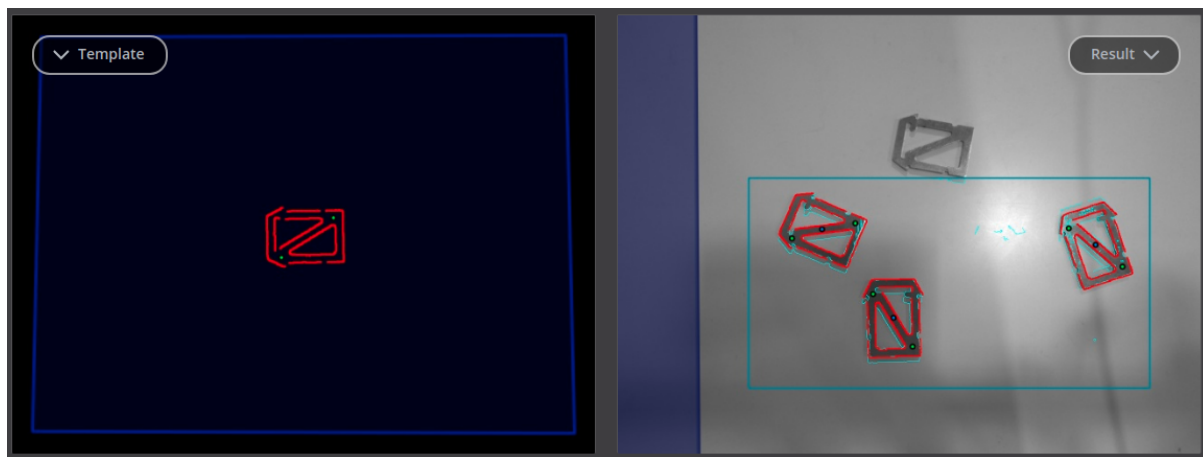
Fig. 7.4: Result image of the SilhouetteMatch component as shown in the Web GUI
