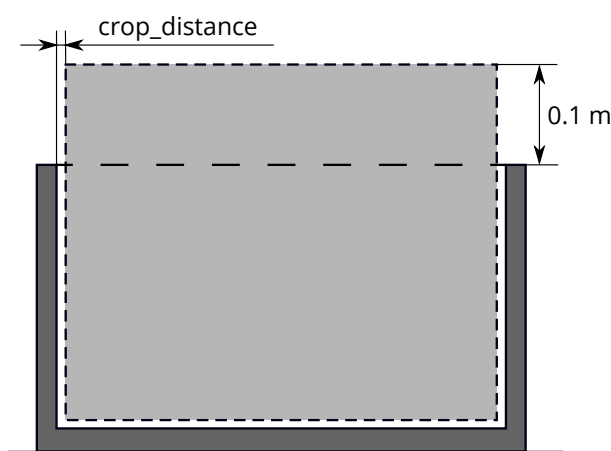
Fig. 7.8: Visualization of the inner volume of a load carrier. Only points which are inside this volume are considered for detections.
