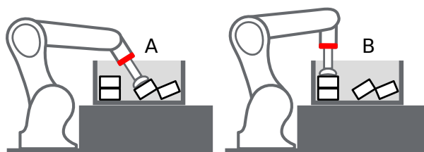
Fig. 7.5: Case A would be marked as collision only if check_flange is true, because the robot's flange (red) is inside the load carrier. Case B is collision free independent of check_flange .
