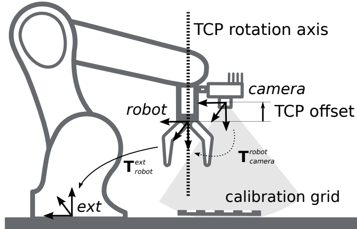
Fig. 6.17: In case of a 4DOF robot, the TCP rotation axis and the offset from the TCP to the camera coordinate system must be provided. In the illustrated case, this offset is negative.
