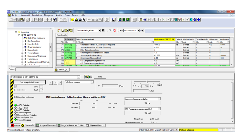
STARTER control panel
