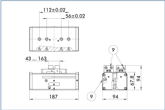
9 For mounting screw connection diagram, see basic version
