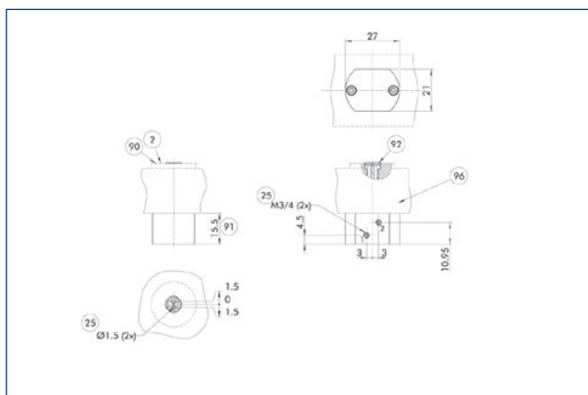
2 Attachment connection
