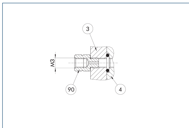
3 Adapter
