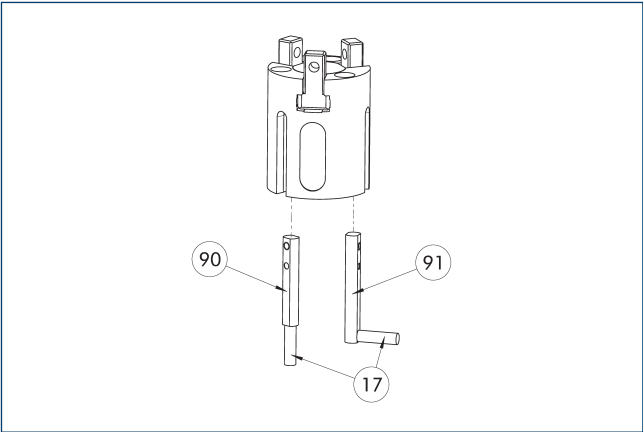
①⑦ Cable outlet ⑨⑩ Sensor MMS 22 PI1-... ⑨① Sensor MMS 22 ..-PI1-...-SA
