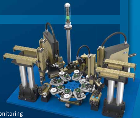
MPG-plus 2-finger gripper for small components with SCHUNK MMS-A analog magnetic sensor and IO-Link Page 84
