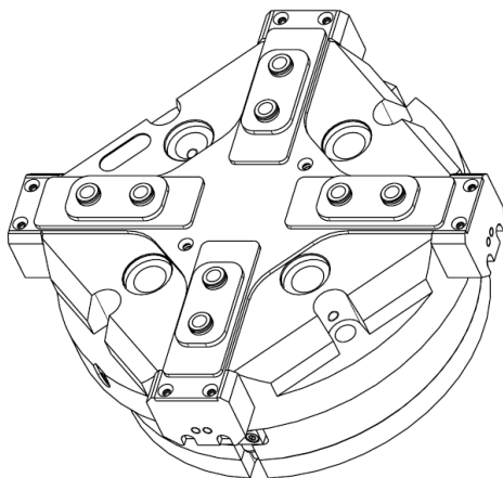
Figure 1: 4-finger gripper with dust cover modification
