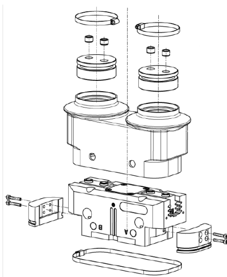
Figure 1: Assembly drawing for a standardized plastic cover
