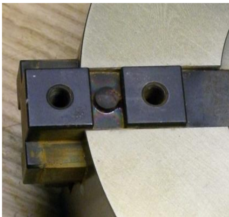
Figure 1: Gripper base jaw without DLC coating after use in corrosive environment
