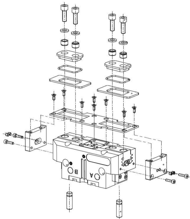
Figure 1: Assembly drawing for mounting of the dust-protection option on a parallel gripper PGN-plus
