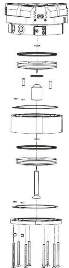
Figure 2: Exploded view of a PZN-plus with option force intensification
