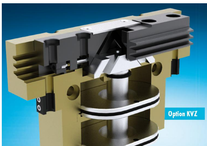
Figure 1: Sectional view of a PGN-plus with option force intensification
