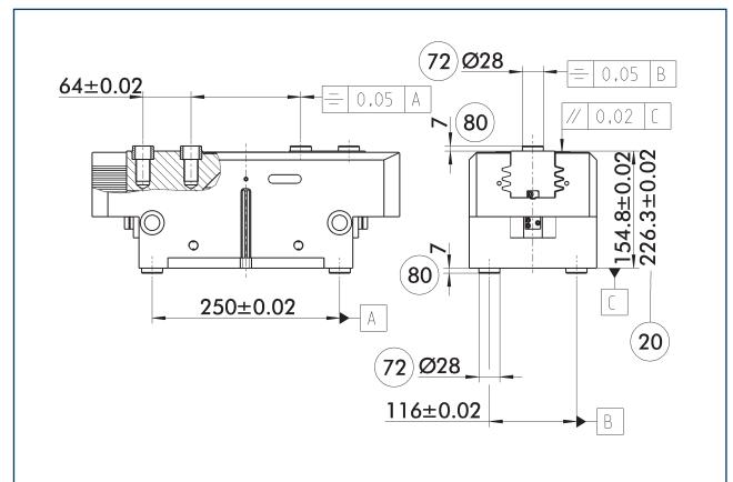
⑧⑩ Depth of the centering sleeve hole in the counter part
