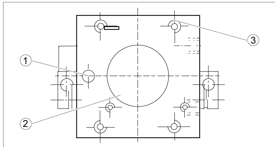
Fastening of the gripper
