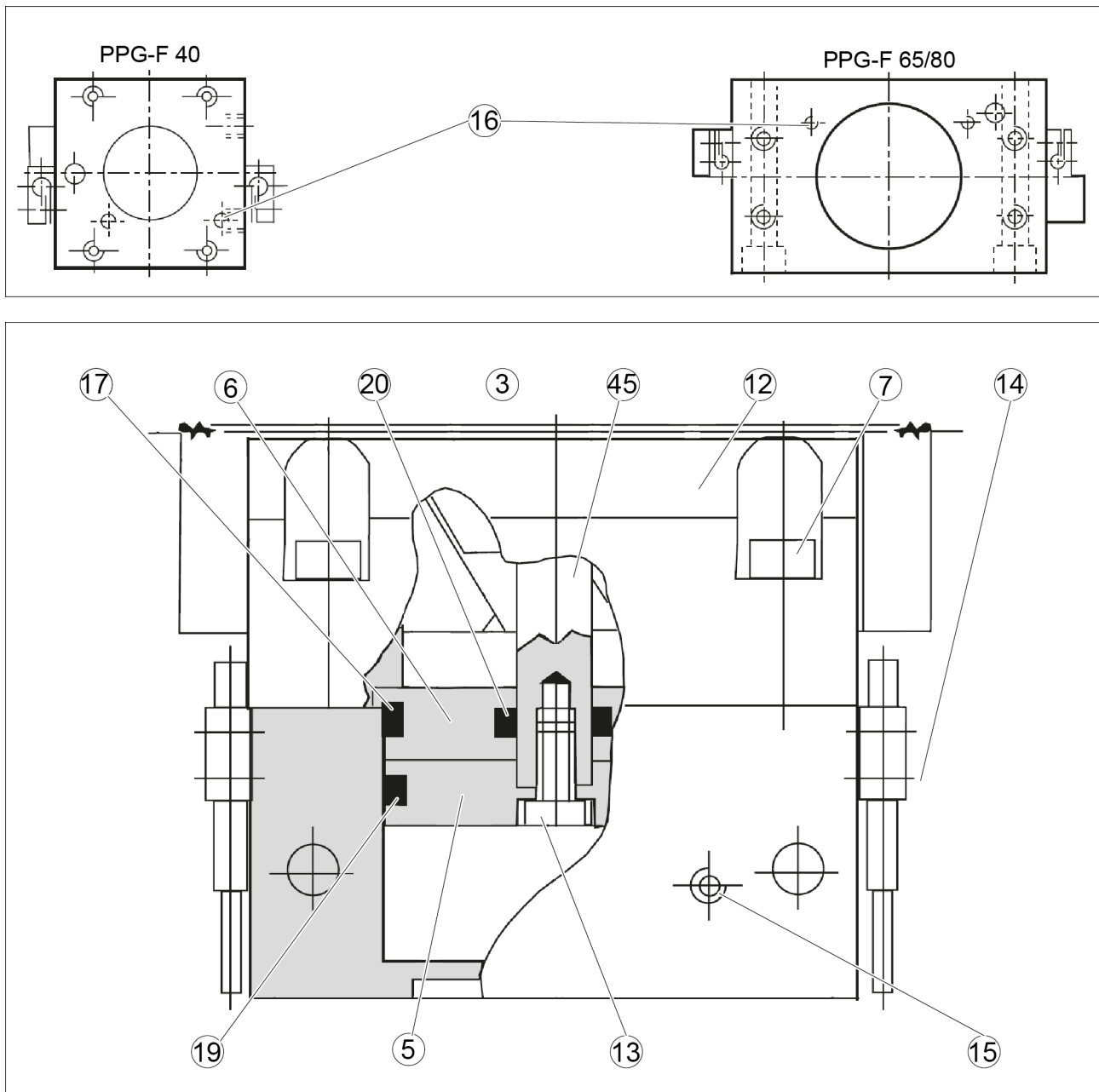
PPG-F without gripping force safety device (in "open" position)
